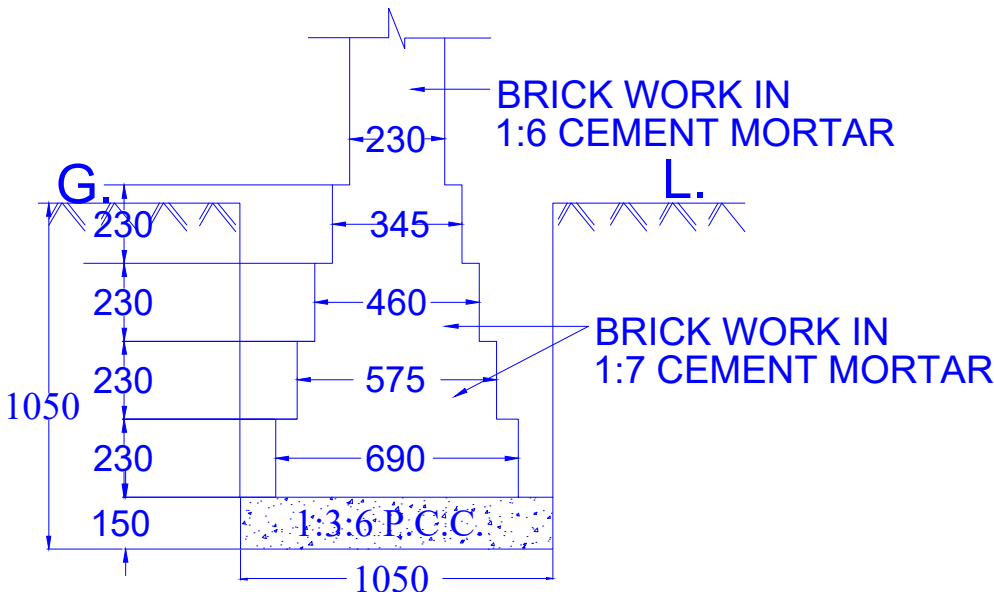
WALL FOUNDATION (NOT FOR SCALE)
