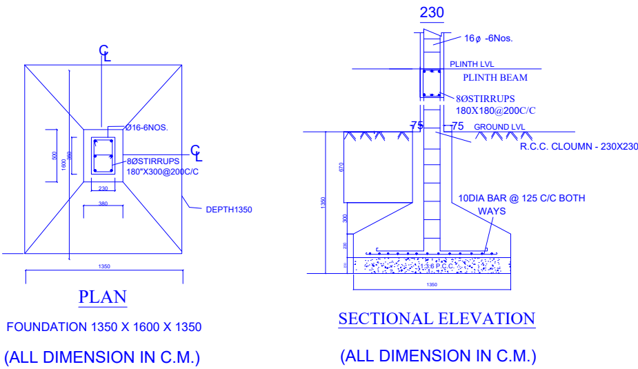
DETAIL OF COLUMN -C (NOT FOR SCALE)
