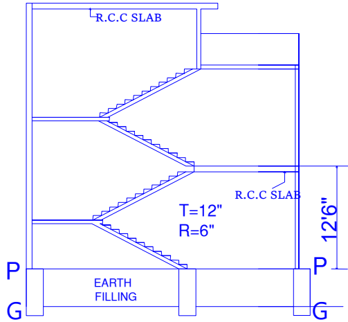
SECTION X-X' (NOT FOR SCALE)
